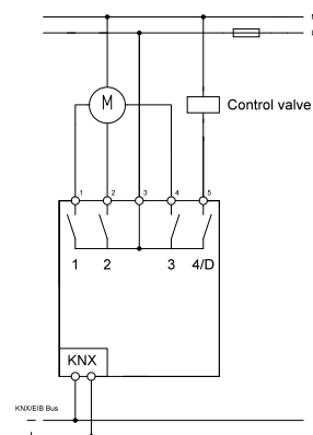
Exemplary circuit diagram AKK-04FC.03 Fan coil
