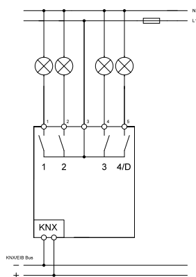
Exemplary circuit diagram AKK-04FC.03 Switching Actuator
